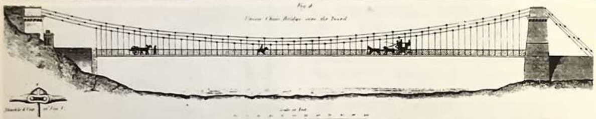
Designed by Captain Samuel Brown R.N. the Union Chain Bridge, 4 miles upstream from Berwick-on-Tweed is the oldest surviving suspension bridge in Britain still carrying vehicles. For the five years prior to Telford's Menai Bridge (1826) it was the longest bridge span in the western world.
