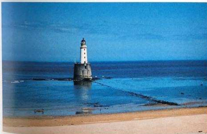
[99] Rattray Head Lighthouse, 1895. The first to be constructed with a fog-horn and signal room beneath its tower.
