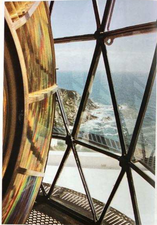
[96] Mull of Kintyre Lighthouse, 1822. Note the later adoption of Alan's inclined astragals, and continuing use of Charles's equiangular prisms.
