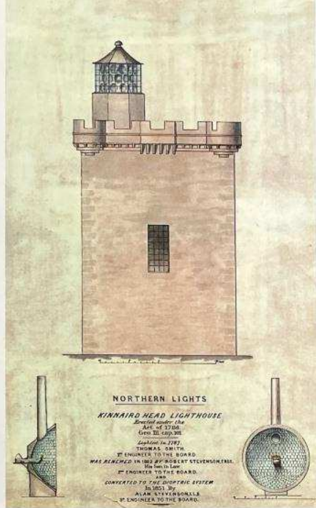
[5] Kinnaird Head Lighthouse and reflector lamp.
