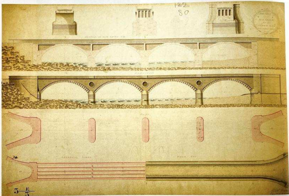
[35] Marykirk Bridge, Kincardineshire, 1811. Robert's first major bridge. Note his use of hollow spandrels for lightness and strength.
