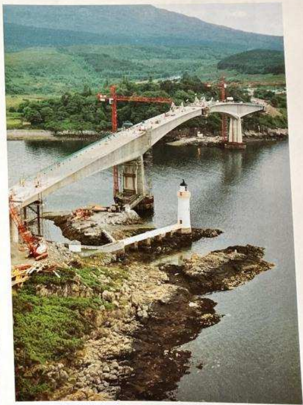
[64] Kyleakin Lighthouse, [1857] of Gavin Maxwell fame and Skye Bridge nearing completion, 1995.
