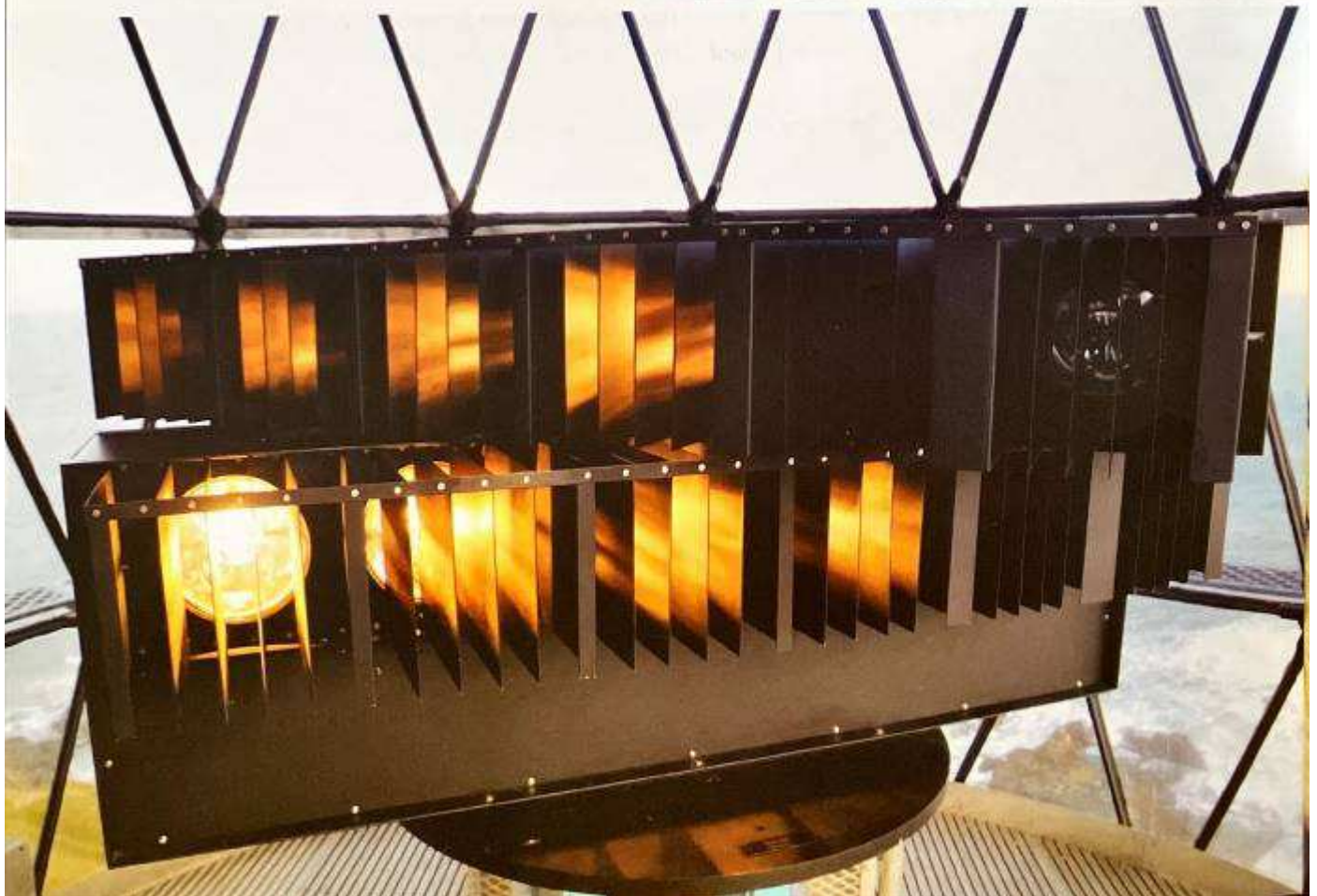
Below: The sealed beam lamp array installed at automation.
