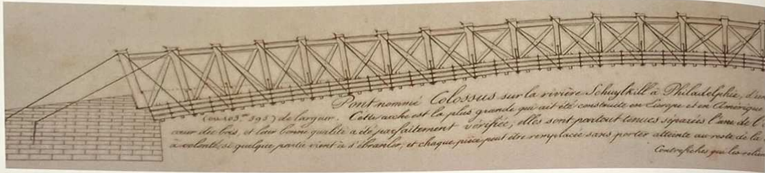
Fig 8 - Wernwag's magnificent timber/iron rod 'Colossus' arch of 340ft span at Philadelphia 1812 (destroyed by fire in 1838)
