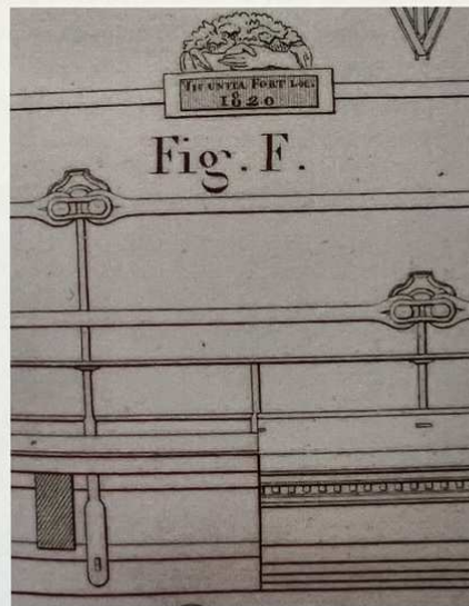
Fig 5 - Union Bridge - mid-span chain, deck and 'VIS UNITA FORTIOR' plaque details [Dupin 1824]
