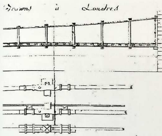
Fig 3 - Brown's works bridge 1813 [Dutens 1819]
