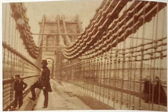
Fig 2 - Menai Bridge's 16 chains each of 5 cross-bolted links
