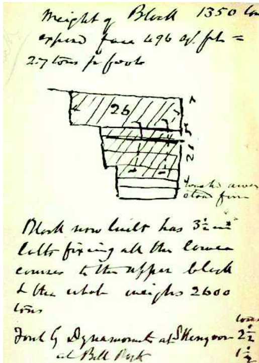
Figure 13. Longitudinal section 1870-72 end [Stevenson] 19 [Plan area about 120 m 2 ]
