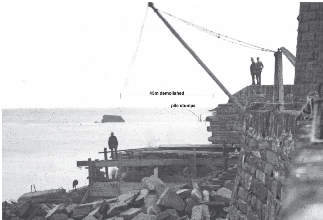
Figure 16. Detached end from North Pier December 1872 ©The Wick Society 17
