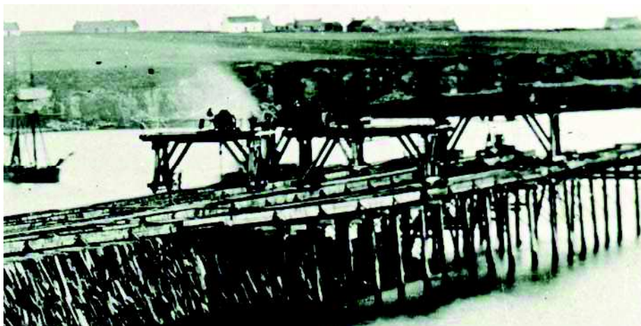
Figure 8. 'Travellers and jennies' in 1865 ©The Wick Society 17
