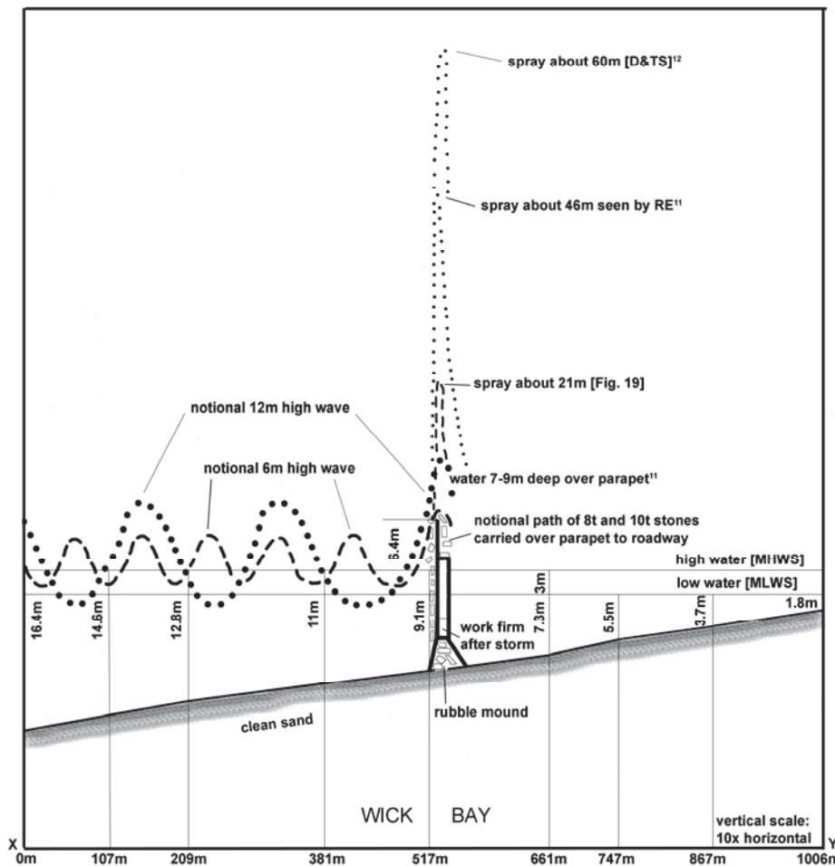
Figure 20. Longitudinal section Wick Bay [X-Y Figure 3] – notional wave action
