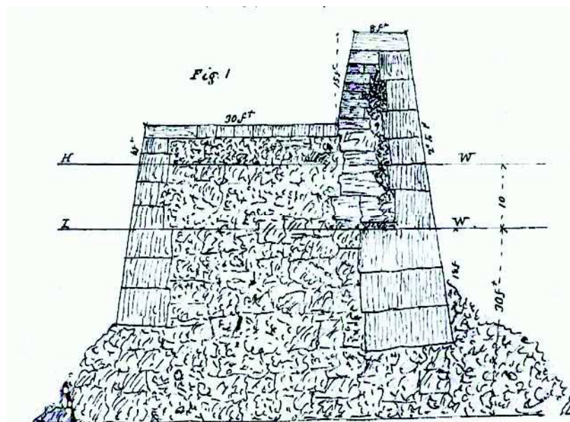
Figure 6. Cross-section as built by 1868 [at 'D' on Figure 3] (Doull 1870) 10
