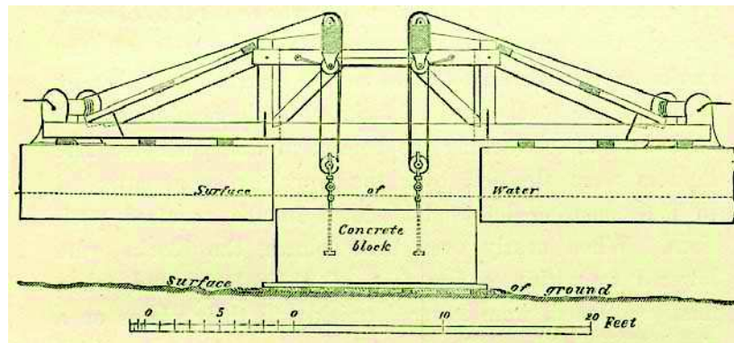
Figure 14. Lowering concrete block from pontoon [Stevenson] 8
