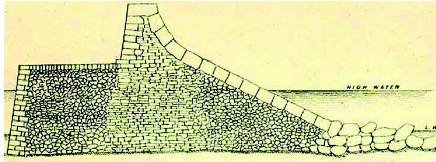
Figure 2. Cross-section of South Pier outer harbour 4
