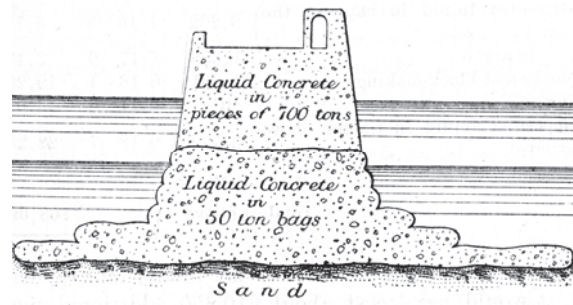
Figure 21. Cay's use of in-situ concrete Aberdeen Harbour North Pier 1874-77
