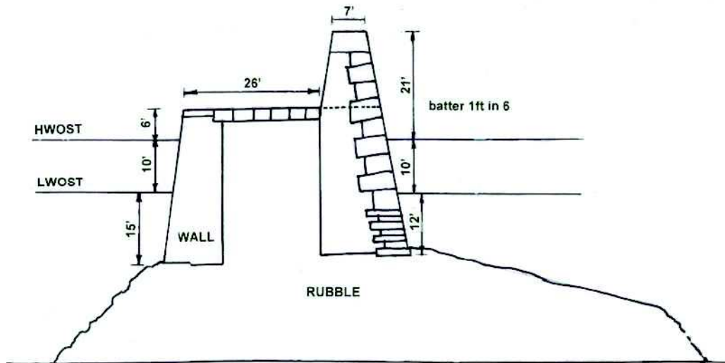
Figure 5. Design cross-section 268 m from shore (1862) 6 NB Tidal range (m) 1984-9: HAT 0.0; MLWS +0.7; MLWN +1.4; MSL +2.0; MHWN +2.8; MHWS +3.5 7
