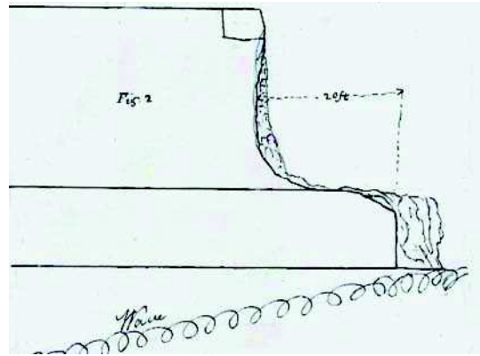
Figure 11. End after February 1870 storm - wave line 12° from face [Doull] 10 Waves at other times parallel to face but curved in plan to 5°-9° at landward end 8
