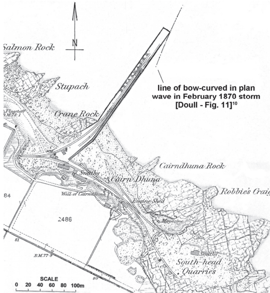
Figure 7. Site layout, quarries, railways in 1872 [Ordnance Survey 1/2500]
